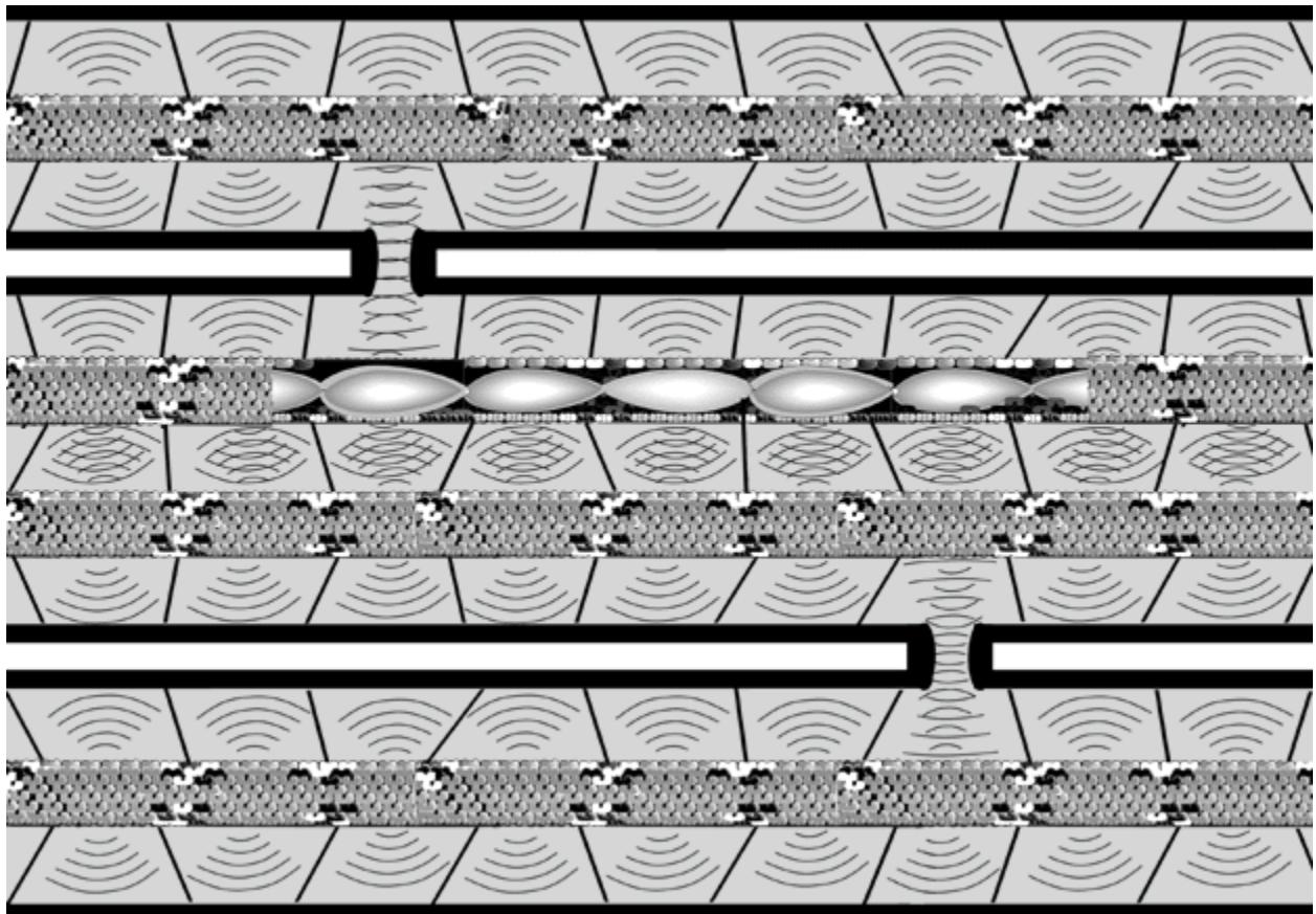
Figure 9. Schematic of proposed quantum coherence in microtubules in three dendrites interconnected by tunneling through gap junctions. Within each neuronal dendrite,
