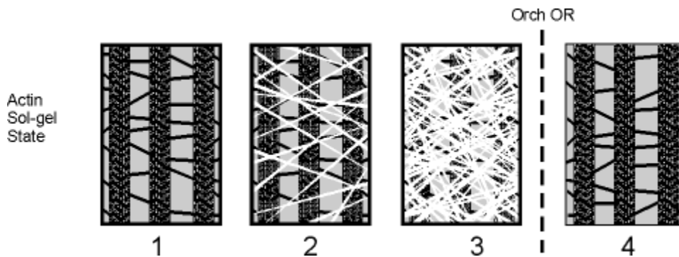
Figure 8. Schematic sequence of phases of actin gelation/quantum isolation (13) alternating with phases of solution/environmental communication (4) surrounding microtubules. Cycles may occur rapidly, e.g., 25 msec intervals (40Hz).
